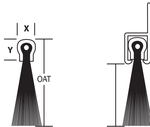
Overall Trim (OAT)
